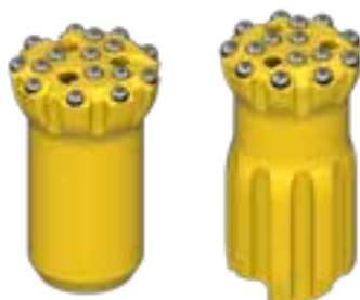
Flat face bit Spherical buttons, standard or heavy duty (HD)
